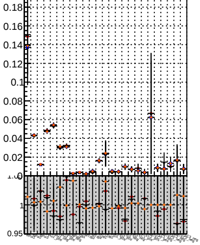
Pileup rate vs \chi^2
