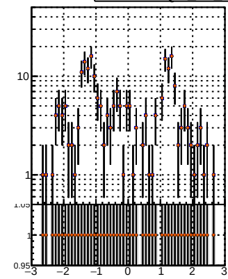
N of reco track vs \eta Legend: BQM TT MS delT-dpdp
