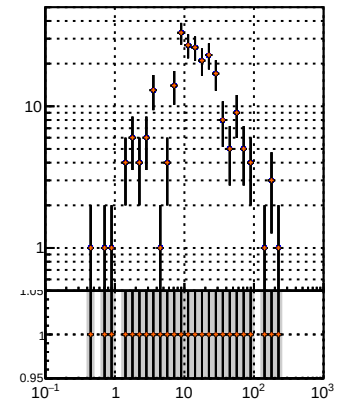
N of reco track vs \eta Legend: BQM TT MS delT-dpdp
