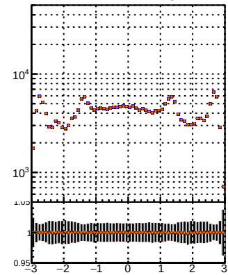
N of reco track vs \eta Legend: \bullet BQM, \square TT, \times MS, \circ delT, \triangle delT-dp2
