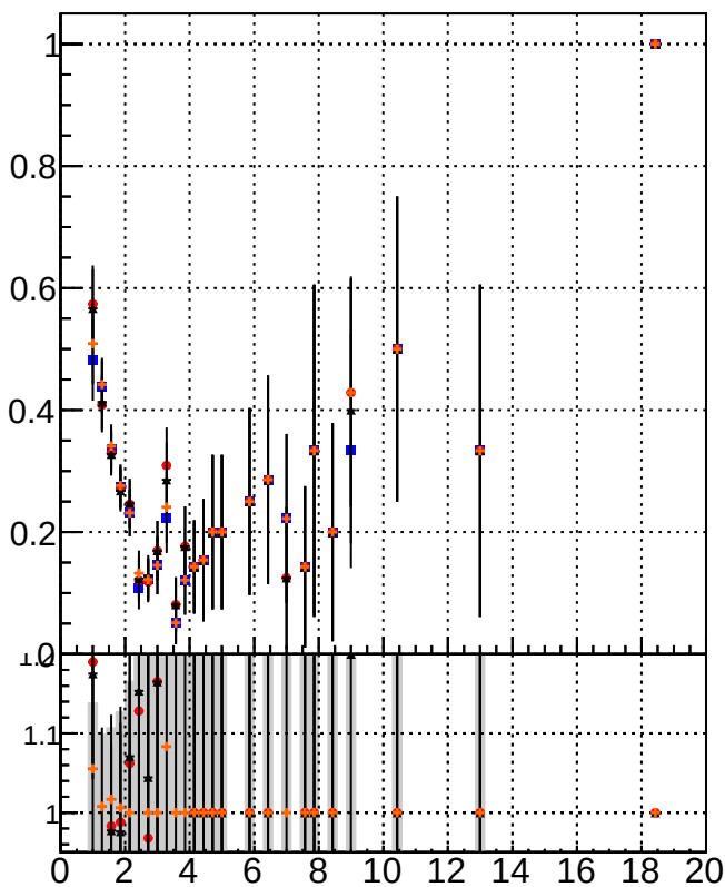
\Delta tracking fake rate vs p\{T\}
