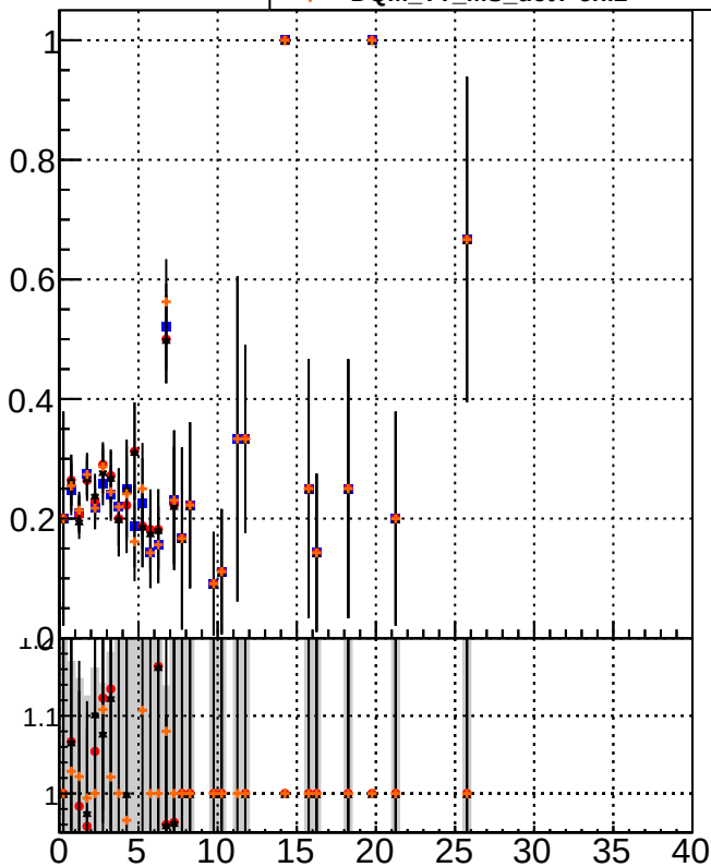
\Delta tracking fake rate
