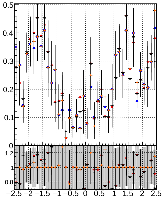
\Delta tracking fake rate vs \eta
