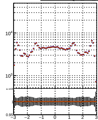
N of reco track vs \eta Legend: \bullet BQM TT MS delT-dp2, \circ BQM TT MS delT-dp2, \square BQM TT MS delT-dp2, \triangle BQM TT MS delT-dp2
