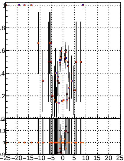
Fake rate vs d D0M TT MS data D0M TT MS data
