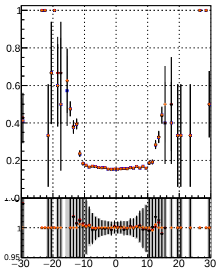
Fake rate vs d D0M TT MS data D0M TT MS data
