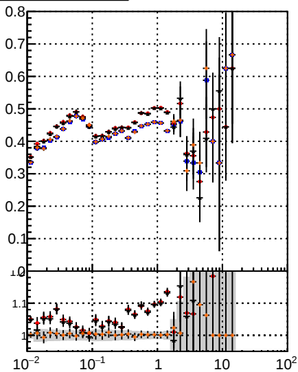
Fake rate vs \sqrt{s} BQM TT MS detT dpdq BQM TT MS detT chi2
