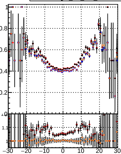
Fake rate vs \sqrt{s} BQM TT MS detT dpdq BQM TT MS detT chi2
