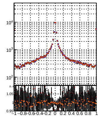
N of reco track vs dxy(PV) Legend: DQM TT MS detT detT-dpda detT-chi2
