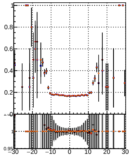
Fake rate vs v DOM TT MS detT dpdq DOM TT MS detT-chi2
