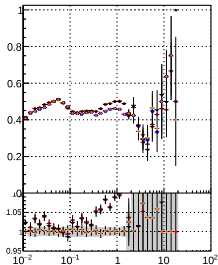
Fake rate vs v DOM TT MS detT detT-dpdaq detT-chi2
