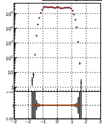
BQM TT MS BQM TT MS N of reco track vs \eta
