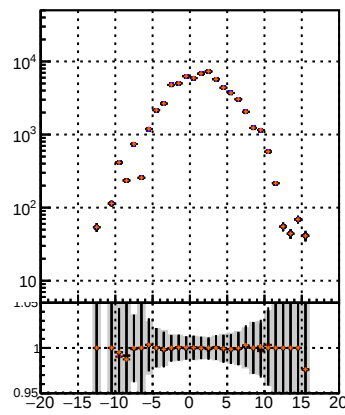
N of associated (recoToSim) loopers tracks vs. sim PV
