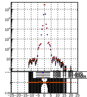
N of reco track vs dxy
