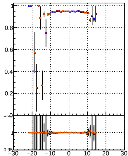
Fake rate vs d Legend: DQM TT MS data09 (blue circles) DQM TT MS det09 (orange circles)
