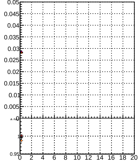
Fake rate vs. \chi^2 for different models and data. Legend: BSM (blue), MS (red), data (black), BSM (orange), MS (green), data (grey).
