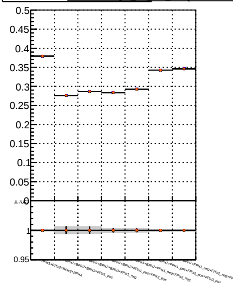
Fake rate vs. Legend: \text{BQM} \parallel \text{MS} \text{ data} (red), \text{BQM} \parallel \text{MS} \text{ det09} (blue), \text{BQM} \parallel \text{MS} \text{ det09} (orange).
