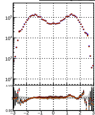
N of reco track vs \eta Legend: BQM (blue circles), TT (red circles), MS (black circles), data09 (orange circles)
