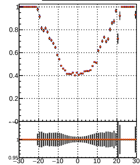
Fake rate vs \sqrt{s} Legend DOM TT MS det0 det01 det09 Line Blue Red Green Black Orange Purple Point Blue Red Green Black Orange Purple
