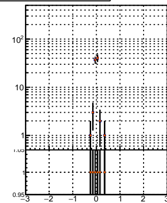
N of associated (recoToSim) duplicate tracks vs \eta Legend: BQM (black), TT (blue), MS (red), S (orange)
