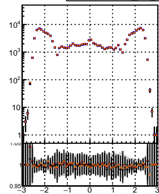
N of reco track vs \eta Legend: BQM (black), TT (blue), MS (red), S (orange)
