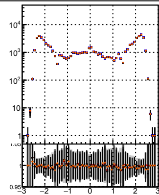
N of associated (recoToSim) tracks vs \eta Legend: BQM (black), TT (blue), MS (red), S (orange)
