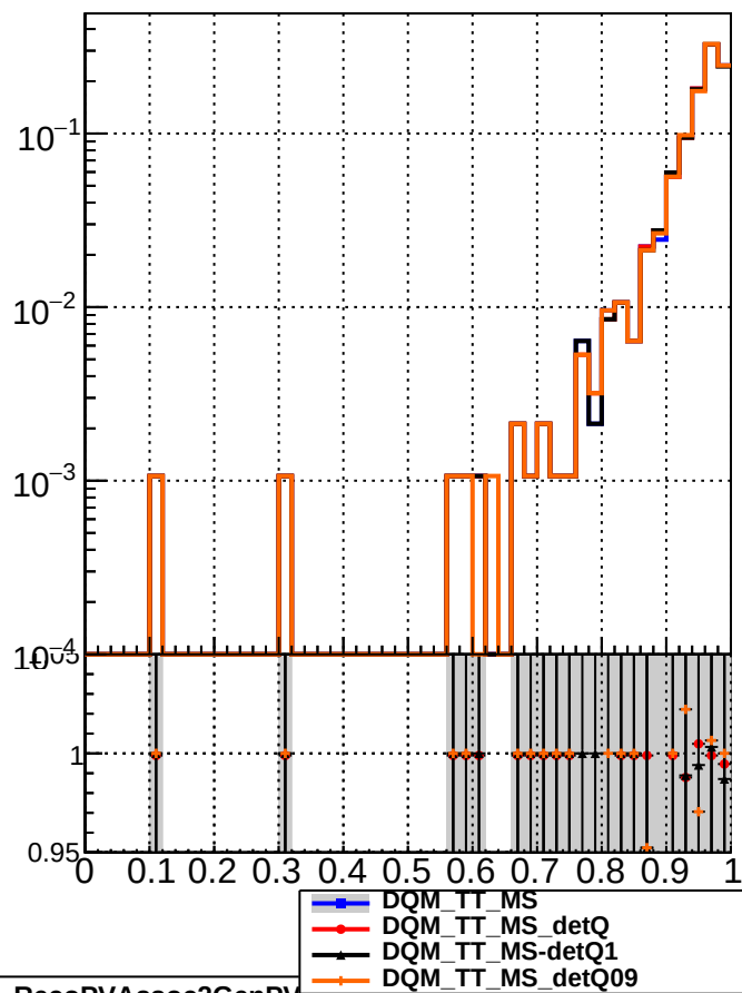
RecoPVAssoc2GenPVMatched_Missing
