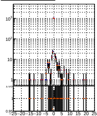
N of reco track vs dxy(PV) vs dxy(PV)
