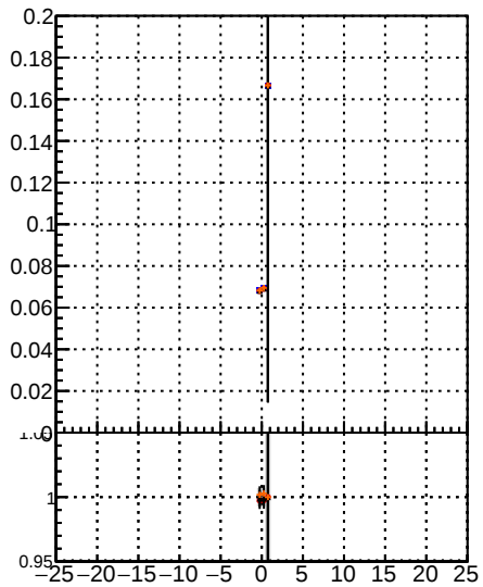
Fake rate vs d BSM data BSM data
