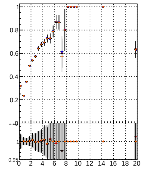
Fake rate vs. \chi^2 for BSM, MS, and data. The legend indicates the color and line style for each data series.
