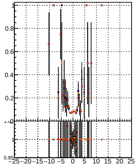
Fake rate vs d BSM MS data BSM MS data
