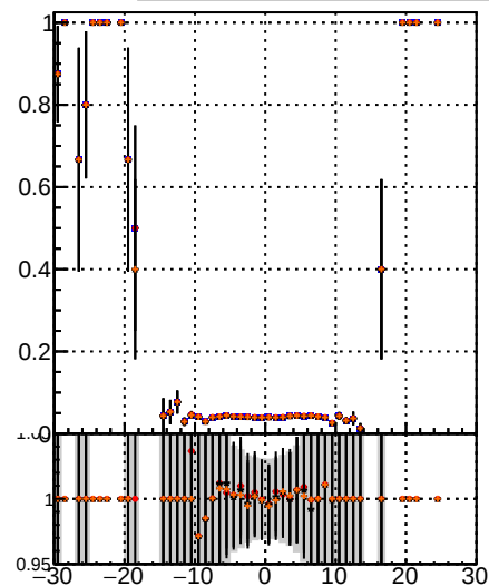
Fake rate vs v Legend: DOM TT MS det0 DOM TT MS det01 DOM TT MS det09
