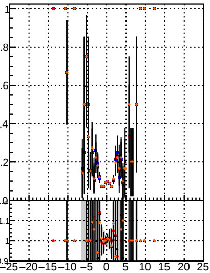
Fake rate vs d BQM MS data BQM MS det09
