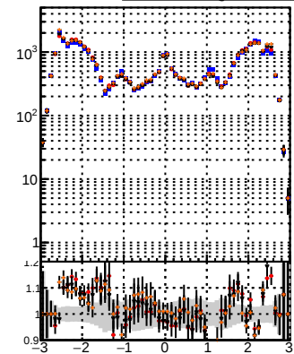
N of reco track vs \eta BQM TT MS data BQM TT MS data09
