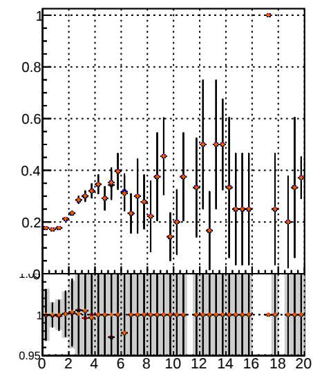
Fake rate vs. \chi^2 for data and MC
