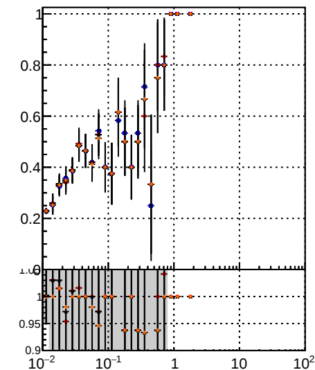
Fake rate vs v Legend: B\bar{B} \rightarrow TT MS det0 (blue squares) B\bar{B} \rightarrow TT MS det01 (orange circles) B\bar{B} \rightarrow TT MS det09 (red triangles) B\bar{B} \rightarrow TT MS det099 (black crosses)
