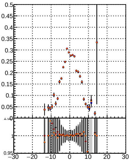
Fake rate vs d MS data MS det09
