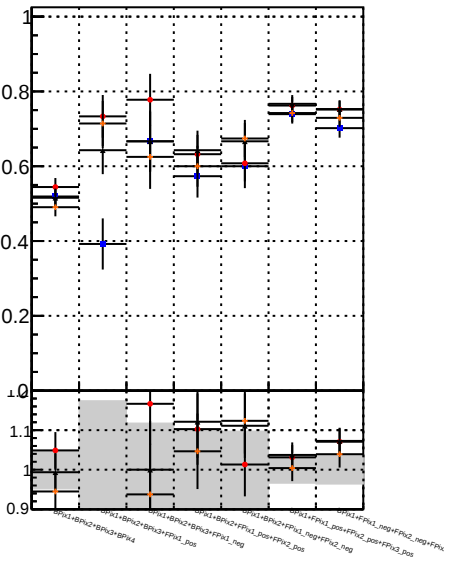
Fake rate vs. BSM IT MS data BSM IT MS data
