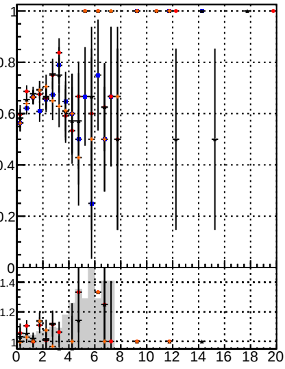
Fake rate vs. BSM IT MS data BSM IT MS data
