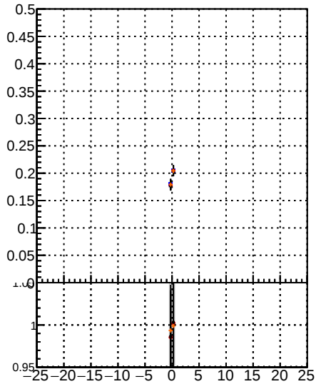
Fake rate vs d Legend: Blue line: BSM Red line: IT Black line: MS Blue dots: data Red dots: data Black dots: data
