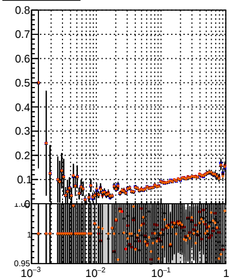
Fake rate vs \sqrt{s} Legend: BQM TT MS det0 BQM TT MS det01 BQM TT MS det09 BQM TT MS det00
