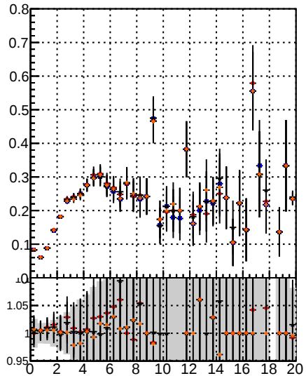
Fake rate vs. BSM MS data BSM MS det09
