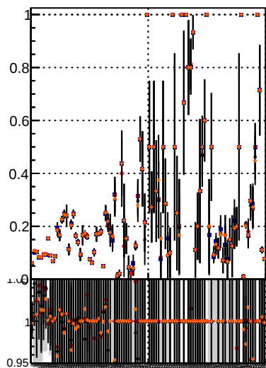
Fake rate vs. BSM MS data BSM MS det09
