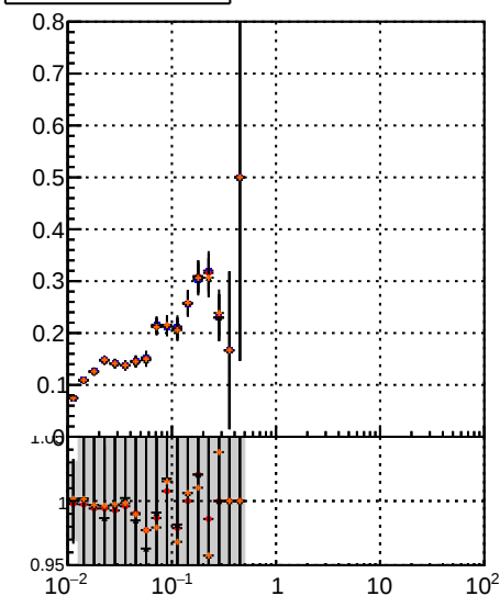
Fake rate vs v Legend: DOM TT MS det0 (blue squares), DOM TT MS det01 (red circles), DOM TT MS det09 (orange triangles), DOM TT MS det09 (green diamonds)
