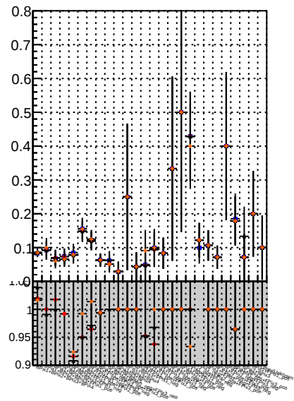
Fake rate vs. BQM MS data BQM MS data
