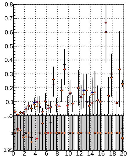
Fake rate vs. BQM MS data BQM MS data
