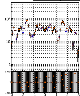
N of reco track vs \eta Legend: BQM TT MS det0 (blue), BQM TT MS det09 (orange), BQM TT MS det09 (red)
