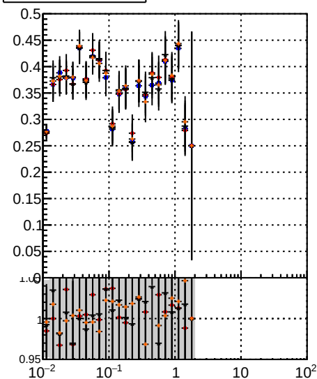
Fake rate vs v \overline{B}0M TT MS det0 \overline{B}0M TT MS det01 \overline{B}0M TT MS det09
