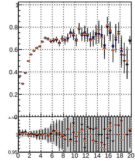
Fake rate vs. \chi^2 for data and MC models.
