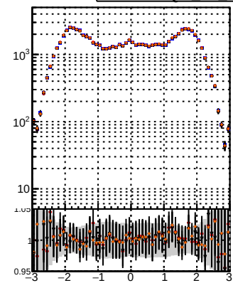
N of reco track vs \eta Legend: BQM (black), TT (blue), MS (red), MS-det09 (orange)
