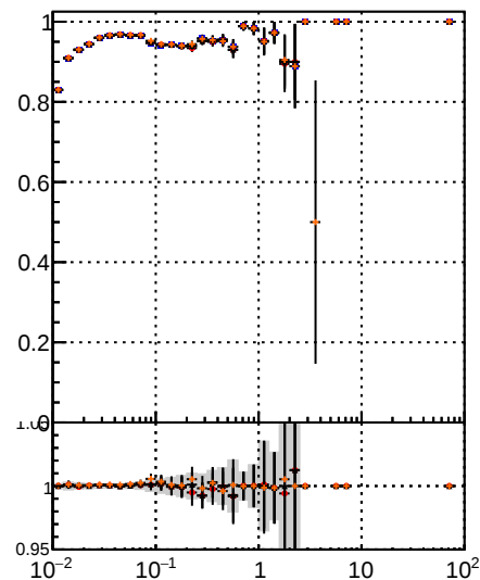
Fake rate vs \sqrt{s} Legend: BQM TT MS det0 (blue squares) BQM TT MS det01 (red circles) BQM TT MS det09 (black crosses) BQM TT MS det099 (orange crosses)
