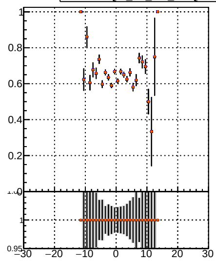
Fake rate vs \sqrt{s} Series Color Shape Line Style MS det0 det01 det09 DOM Blue Square Solid TT MS MS MS DOM Red Circle Solid TT MS MS MS DOM Black Triangle Solid TT MS MS MS DOM Orange Diamond Solid TT MS MS MS DOM Green Star Solid TT MS MS MS DOM Purple Hexagon Solid TT MS MS MS DOM Brown Octagon Solid TT MS MS MS DOM Grey Circle Dashed TT MS MS MS DOM Light Blue Square Dashed TT MS MS MS DOM Light Red Circle Dashed TT MS MS MS DOM Light Green Triangle Dashed TT MS MS MS DOM Light Orange Diamond Dashed TT MS MS MS DOM Light Purple Star Dashed TT MS MS MS DOM Light Brown Hexagon Dashed TT MS MS MS DOM Light Grey Octagon Dashed TT MS MS MS
