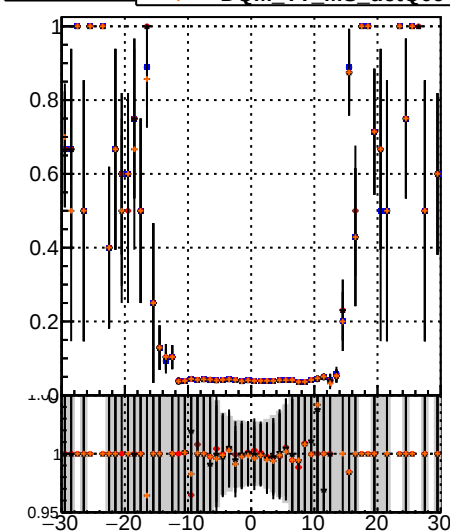
Legend: - \text{BQM} \rightarrow \text{TT} \rightarrow \text{MS} \rightarrow \text{detQ} (blue line with circles) - \text{BQM} \rightarrow \text{TT} \rightarrow \text{MS} \rightarrow \text{detQ1} (red line with circles) - \text{BQM} \rightarrow \text{TT} \rightarrow \text{MS} \rightarrow \text{detQ9} (orange line with circles)
