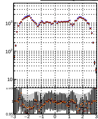
N of reco track vs \eta Legend: BQM (black), TT (red), MS (blue), data (orange)
