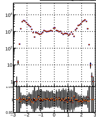
N of reco track vs \eta Legend: BQM (black), TT (blue), MS (red), det0 (orange)
