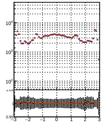
N of reco track vs \eta BQM TT MS data09 BQM TT MS data09 BQM TT MS data09
