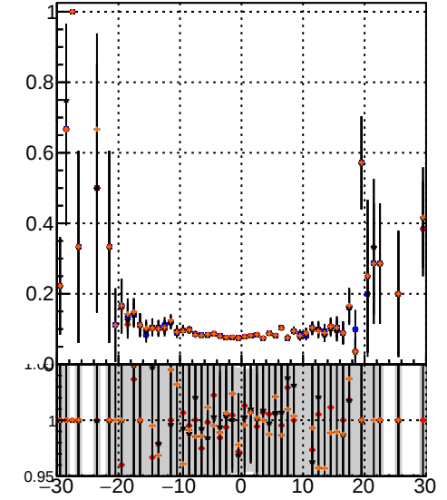
Efficiency vs. sim PV z Legend: DQM_TT_MS (blue circles) DQM_TT_MS_detQ (red circles) DQM_TT_MS_detQ1 (black circles) DQM_TT_MS_detQ09 (orange circles)
