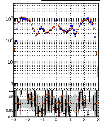
N of reco track vs \eta Legend: BQM (blue circles), TT (black circles), MS (red circles), data09 (orange circles)
