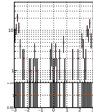
N of associated (recoToSim) duplicate tracks vs \eta BQM TT MS det0 BQM TT MS det009
