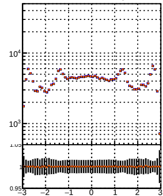
N of reco track vs \eta BQM TT MS det0 BQM TT MS det009
