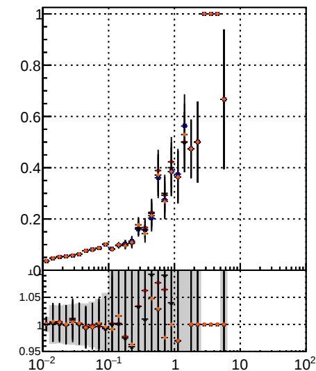
Fake rate vs v BQM TT MS det0 BQM TT MS det01 BQM TT MS det09
